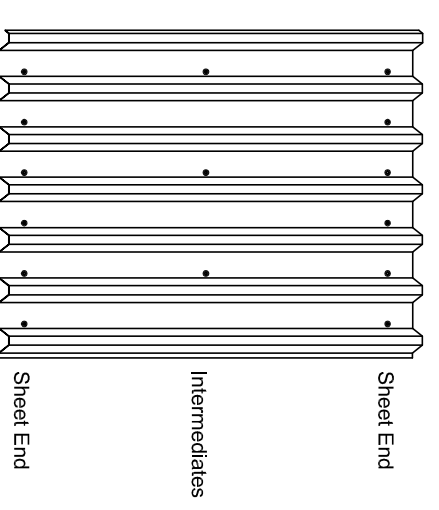
Liner Sheet Fixing Arrangement N/S
