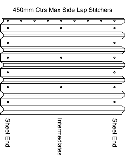
Top Sheet Fixing Arrangement N/S
